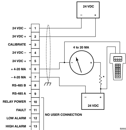
Figure 9—Eclipse Detector Wired for Isolated 4-20 mA Current Output (Sinking)
