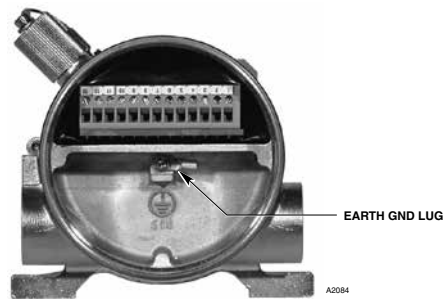
Figure 4—Terminal Strip Located Inside Wiring Compartment
