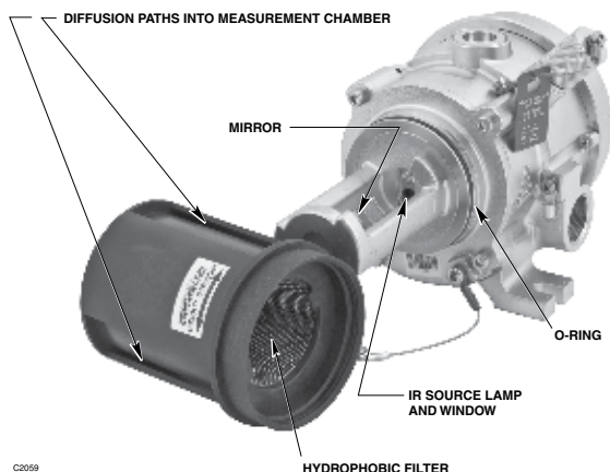
Figure 22—PointWatch Eclipse with Baffle Removed
