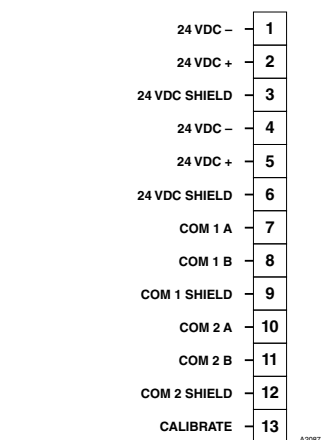
Figure 14—Wiring Terminal Identification for Eagle Quantum Premier Eclipse
