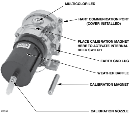
Figure 19—PointWatch Eclipse
