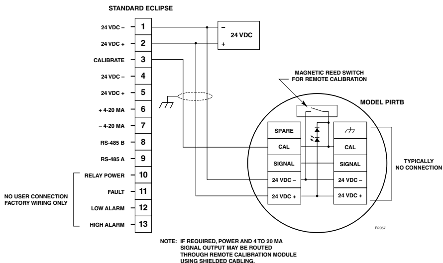
Figure 17—Remote Calibration Module Wired to Standard PointWatch Eclipse
