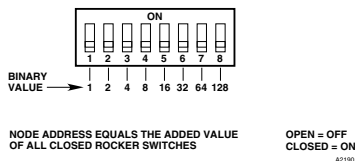
Figure H-1—PIRECL Address Switches
