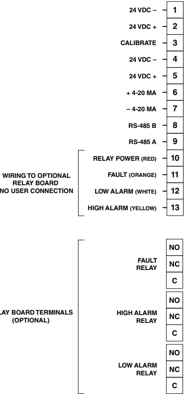
Figure 6—Wiring Terminal Identification for Standard Eclipse with Relays
