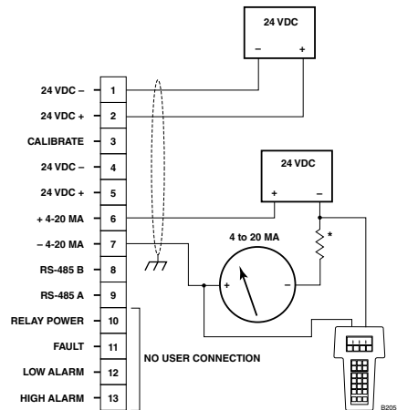
Figure 10—Eclipse Detector Wired for Isolated 4-20 mA Current Output (Sourcing)
