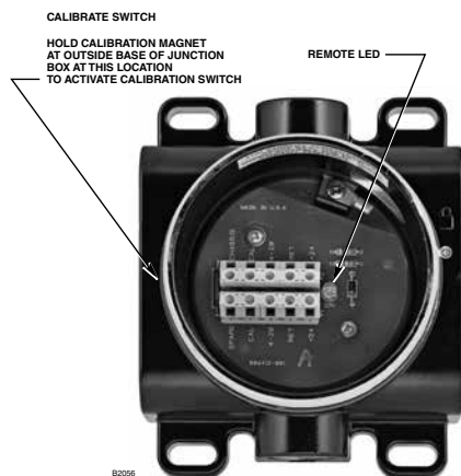
Figure 16—Remote Calibration Switch and LED in Optional Det-Tronics PIRTB Termination Box
