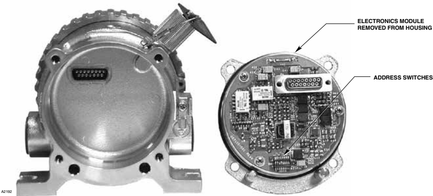
Figure H-2—Location of PIRECL Address Switches
